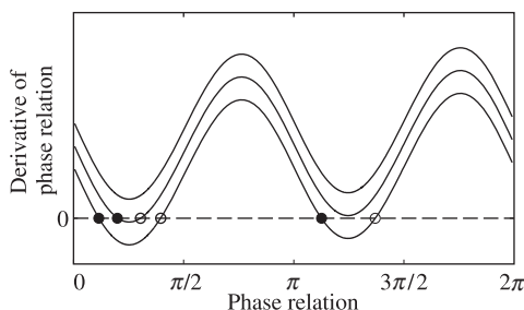
Figure 1. Schematic representation of the extended HKB equation attractor landscape. Each curve depicts the derivative of phase relation ( y -axis) throughout its state space ( x -axis) given three different values for the symmetry-breaking parameter (lower, middle, and upper curves). Stable points are represented by filled circles and unstable ones by open circles. The phase relation dynamics changes from multistable (lower curve) to monostable (middle curve) and eventually metastable (upper curve).
