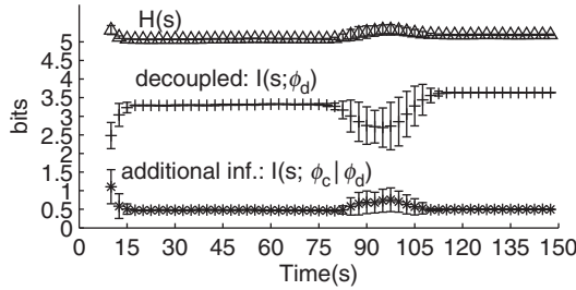
Figure 13. Information-theoretic measures for the agent’s controller with and without the modulation \phi \rightarrow s . All measures represent the mean over 20 trials and error bars their standard deviation. On average, the agent’s sensor entropy H(s) remains around 5 bits. Under open-loop, the mutual information between the decoupled agent’s controller and its sensor I(s; \phi_d) stays at \approx 3.3 bits while the agent is approaching the centre of the environment (time in seconds is represented on the x -axis) and slightly increases to \approx 3.6 when the agent is moving around the centre of the environment. The controller of the coupled agent carries 0.5 bits of additional information about the sensor that is not present in the controller of the decoupled agent, shown by I(s; \phi_c | \phi_d) .
