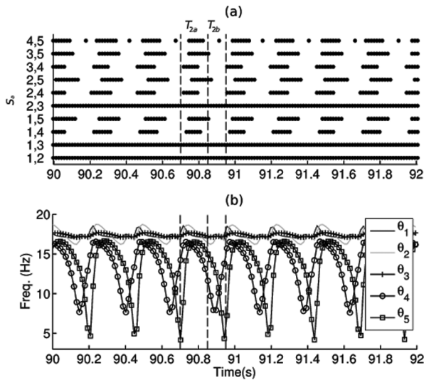
Figure 7. (a) shows the synchronization dynamics S_0 underlying SM_{T_2} . Each black point corresponds to a moment of synchrony between the pair of oscillators depicted in the y -axis. (b) shows the frequency dynamics of all five oscillators (see legend).
