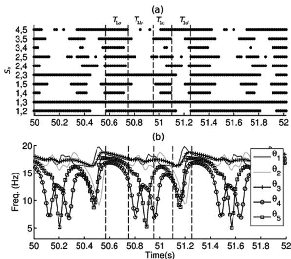
Figure 6. (a) shows the synchronization dynamics for the multivariate time series S_a underlying SM_{T_1} . The y-axis contains all pairs of oscillators and each black point in the image corresponds to a moment of synchrony. (b) shows the frequency dynamics of all five oscillators (see legend).
