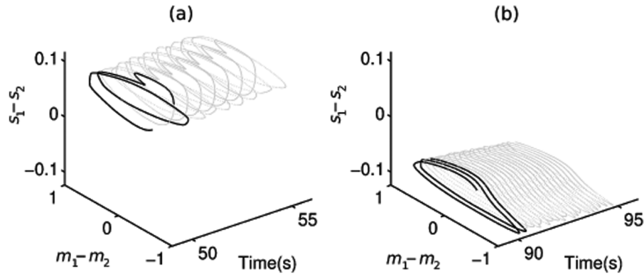
Figure 2. (a) and (b) show the sensorimotor dynamics SM(t) = (s_1(t), s_2(t), m_1(t), m_2(t)) during T_1 and T_2 . The x-axis shows the time in s, the y-axis shows the difference in activation of the right and left motors ( m_r - m_l ) and z shows the difference in activation of the right and left sensors ( s_1 - s_2 ). The black trajectories in both images highlight the first 600 ms of each time-window.
