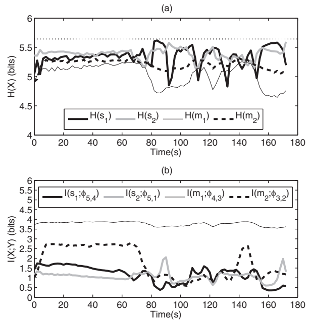
Figure 8. (a) shows the entropy ( y -axis) of each sensorimotor component (see legend) during the agent's lifetime ( x -axis). Straight dotted line at the top ( y = 5.64 bits) represents the maximum possible value for the entropies. (b) shows the mutual information between four combinations of components from SM and P , namely I(SM(s_1); P(\phi_{5,4})) , I(SM(s_2); P(\phi_{5,1})) , I(SM(m_1); P(\phi_{4,3})) and I(SM(m_2); P(\phi_{3,2})) , see legend.
