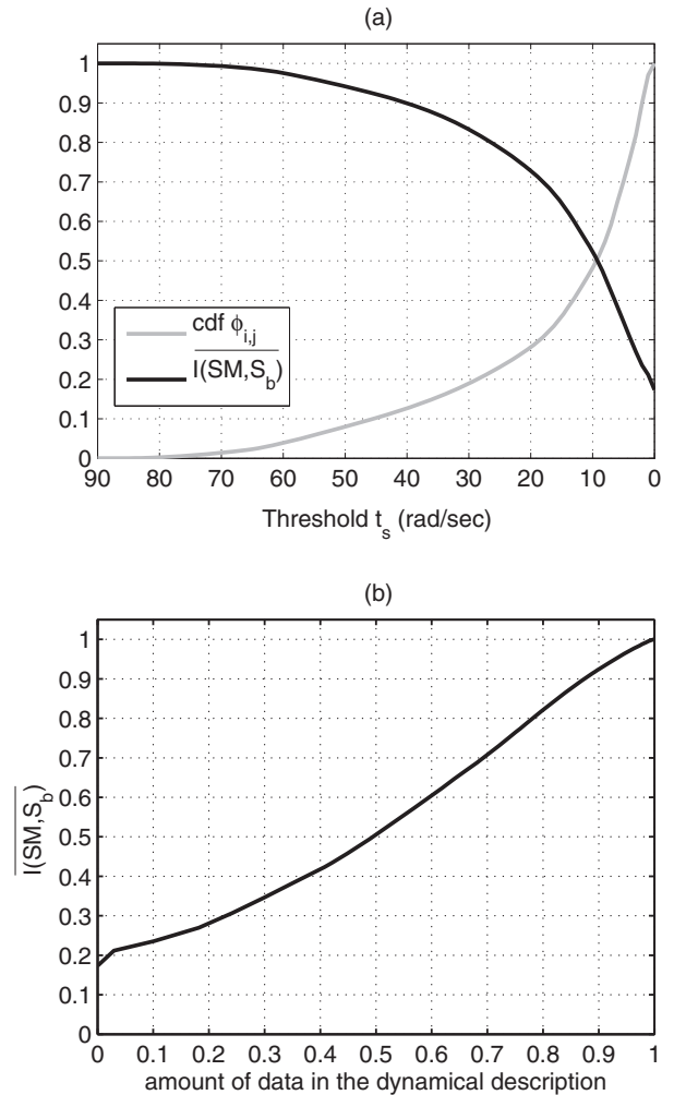
Figure 10. Mutual information between the phase relations and the sensorimotor dynamics for different values of t_s . The black line in (a) shows how \overline{I(SM,S_b)} changes as the threshold t_s decreases (notice inverted x-axis). The values of \overline{I(SM,S_b)} are normalized in [0,1] with 1 representing the maximum \overline{I(SM,S_b)} = 1.50 bits. The gray line shows the cumulative function distribution (cdf) of \dot{\phi}_{i,j} . It represents the quantity of \dot{\phi}_{i,j} greater than a t_s ; for instance, 20% of \dot{\phi}_{i,j} are greater than 30 rad/s. (b) shows how \overline{I(SM,S_b)} (y-axis) changes in relation to the amount of data in the dynamical descriptions (i.e. the quantity of phase relations considered to be synchronized), where the maximum value 1 (x-axis) represents the complete description and smaller values represent reduced descriptions obtained by decreasing the threshold. For instance, when S_b contains 0.3 of the dynamics of phase relations (the other 0.7 are desynchronized oscillations) then \overline{I(SM,S_b)} = 0.34 ; i.e. 30% of the most synchronized oscillations carry 34% of the total amount of information about sensorimotor dynamics; the other 70% of oscillations, which are desynchronized, carry the remaining 66% of the total information.
