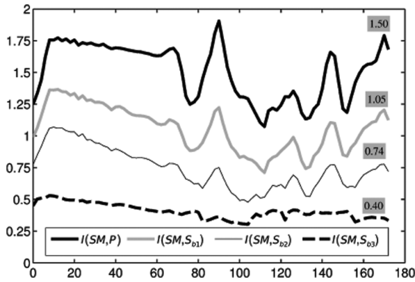
Figure 9. Mean mutual information between all 40 pairs of sensorimotor and phase relation components. I(SM,P) shows the maximum mutual information in the phase relations throughout the trial (see time in the x-axis). I(SM,S_{b1}) , I(SM,S_{b2}) and I(SM,S_{b3}) represent the mutual information from three reduced description with thresholds t_s = 18 , t_s = 9 and t_s = 3 rad/s respectively. The lower the t_s the less information present in the reduced descriptions. The numbers highlighted with gray background at the end of each line represent the mean mutual information over the whole trial, namely \overline{I(SM,P)} = 1.50 , \overline{I(SM,S_{b1})} = 1.05 , \overline{I(SM,S_{b2})} = 0.74 , and \overline{I(SM,S_{b3})} = 0.40 bits.
