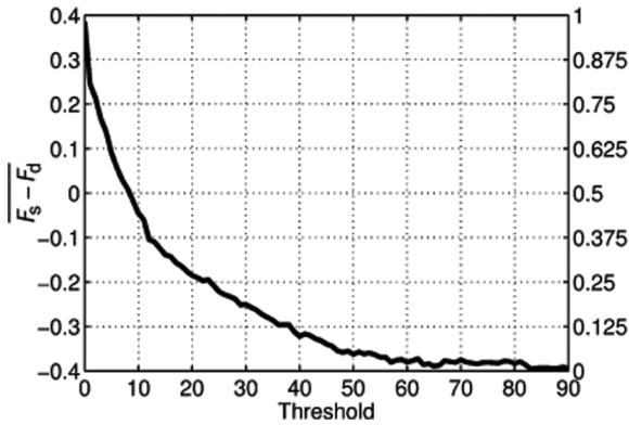
Figure 12. Mean of fitness difference \overline{F_s - F_d} (y-axis on the left) for different thresholds t_s (x-axis). Positive values indicate that desynchronization is more relevant than synchronization for the generation of functional sensorimotor coordination. The y-axis on the right side represents \overline{F_s - F_d} rescaled to [0,1] . When the rescaled \overline{F_s - F_d} is 0.5, for instance, both types of oscillations are equally relevant. The rescaled \overline{F_s - F_d} works as an index of relevance for desynchronous oscillations, where 0 indicates no relevance and 1 maximum relevance.
