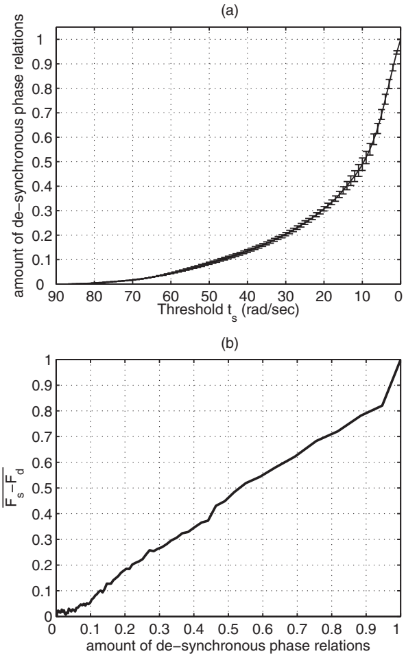
Figure 13. (a) shows how the quantity of desynchronous phase relations changes (y-axis) for different thresholds (x-axis). Bars represent the standard deviations. Near 50% of the phase relations have their derivative \dot{\phi}_{i,j} < 10 rad/s. (b) shows how the relevance of desynchronized oscillations, i.e. \overline{F_s - F_d} rescaled to [0, 1] , changes in relation to the quantity of phase relations considered desynchronized (x-axis).
