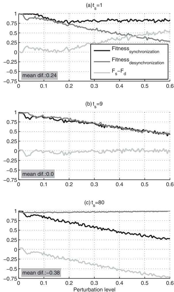
Figure 11. Agent's fitness (y-axis) for different levels of perturbations \alpha (x-axis) and thresholds t_s = 1 (a), t_s = 9 (b), and t_s = 80 (c). Black and dark-gray lines show the fitnesses of the agent when perturbation is applied to synchronous and desynchronous oscillations, respectively (see legend). The light-gray line is the fitness difference F_{\text{synchronization}} - F_{\text{desynchronization}} (see legend). The numbers highlighted with a gray background show the mean of the fitness difference over all perturbation levels. This mean will be referred to as \overline{F_s - F_d} .
