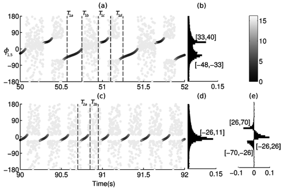
Figure 5. Synchronization dynamics for \theta_1 and \theta_5 ( S_b(\phi_{1,5}) ) underlying sensorimotor regimes SM_{T_1} (a) and SM_{T_2} (c). The relation \phi_{1,5} is shown in the y-axis and time in the x-axis. The color bar shows \dot{\phi}_{1,5} , where the darker the color the lower the derivative. Dashed lines highlight the small time-windows T_{1a} , T_{1b} , T_{1c} and T_{1d} (a) and T_{2a} and T_{2b} (c). These images were generated for t_s = 15 rad/s. The disperse gray dots represent phase relations that were shuffled. The derivative \dot{\phi}_{1,5} is greater than 15 rad/s during the entire time-windows T_{1b} and T_{2b} . (b) and (d) show the density distribution of each regime of phase relation. (e) shows the difference on the density distributions.
