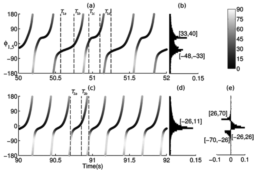
Figure 3. Phase relations between \theta_1 and \theta_5 ( P(\phi_{1,5}) ) underlying sensorimotor regimes SM_{T_1} (a) and SM_{T_2} (c). The relation \phi_{1,5} is shown in the y-axis and time in the x-axis. The color bar shows \dot{\phi}_{1,5} in rad/s, where the darker the color the lower the derivative. For ease of description we highlight four small time-windows during T_1 : T_{1a} , T_{1b} , T_{1c} and T_{1d} of 180, 200, 150 and 150 ms, respectively (see dashed lines in (a)) and other two time-windows during T_2 : T_{2a} and T_{2b} of 150, 100 ms, respectively (see dashed lines in (c)). Note that the x-axis depicts only 2 s ([50,52]) rather than 5 s ([50,55]). While underlying SM_{T_1} the phase relation \phi_{1,5} has two regions where it slows down (see T_{1a} and T_{1c} ); underlying SM_{T_2} it has only one around 0 degrees (see T_{2a} ). This difference can be seen by the peaks of density distributions of \phi_{1,5} shown in (b) and (d). These distributions were generated for the two-second time-windows [50,52] s and [90,92] s, respectively. (e) shows the difference between the density distributions shown in (b) and (d).
