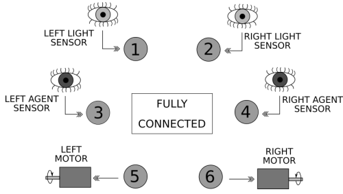
Figure 2: Agent's controller
